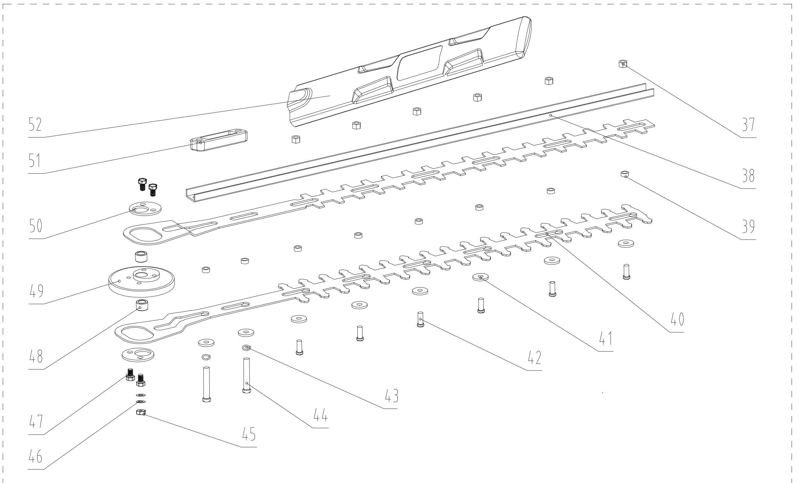
Hedge Trimmer
